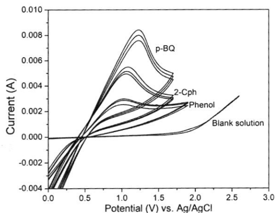
Fig. 4. Cyclic voltammograms of diamond composite electrodes in an aqueous solution of 0.1 M sulfuric acid containing 200 mg/L p -BQ, 2-Cph or phenol. Scan rate 100 mV/s and 25 °C temperature and pH 3.
