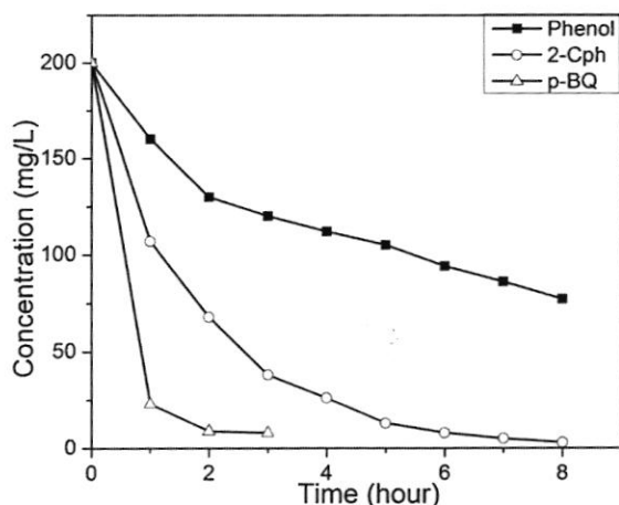
Fig. 6. Electrochemical degradation of 200 mg/L p -BQ, 2-Cph, and phenol in aqueous solution of 0.25 M Na 2 SO 4 as supporting electrolyte at pH 3 and 25 °C temperature.
