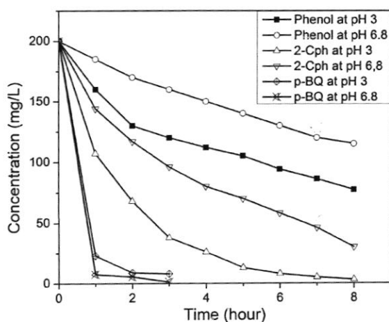
Fig. 7. Electrochemical degradation of 200 mg/L of p -BQ, 2-Cph, and phenol in different pH solutions (pH 3 and pH 6.8) with 0.25 M Na 2 SO 4 as supporting electrolyte and 25 °C temperature.
