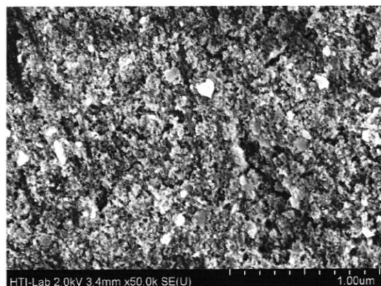
Fig. 1. Scanning electron microscopy (SEM) image for diamond composite electrode. The scan was performed at high magnification ( \times 50,000 times) with image resolution at 1.00 μm.
