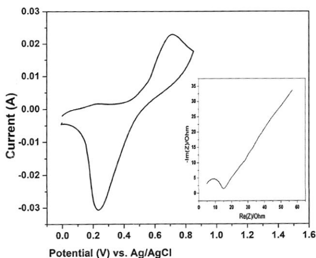
Fig. 3. Cyclic voltammogram of diamond composite electrode in aqueous solution of 0.25 M \text{H}_2\text{SO}_4 containing 5 mM \text{K}_4\text{Fe}(\text{CN})_6 at 100 mV/s scan rate and 25 °C. Inset is the Nyquist plot of the electrode in same aqueous solution at zero potential vs. Ag/AgCl.
