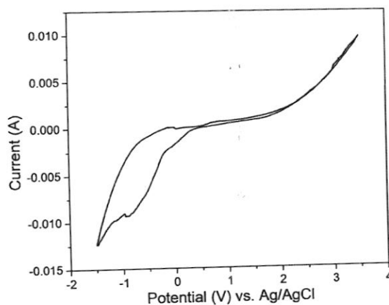
Fig. 2. Cyclic voltammetry of diamond composite electrodes in an aqueous solution of 0.25 M H_2SO_4 . Scan rate 100 mV/s and 25 °C temperature.
